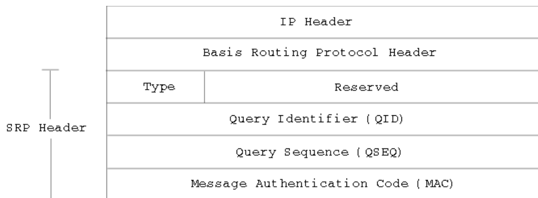
Figure 4. SRP Packet Header: the input to the keyed hash function is the IP header, the header of the basis protocol, and the shared secret.
