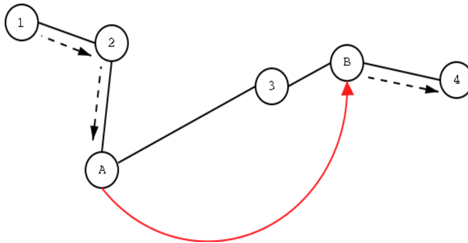
Figure 1. A wormhole attack performed by colluding malicious nodes A and B.
