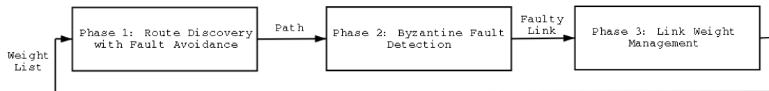
Figure 7. The three phases of the protocol operate in sequence and each one receives the output of the previous as input.
