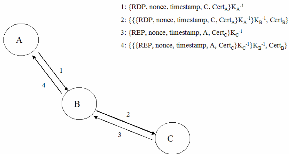
Figure 2. Route discovery in the ARAN protocol: Messages 1 and 2 are broadcasted, while 3 and 4 are unicasted ( \{M\}K_N^{-1} denotes a signature on message M generated by private key K_N^{-1} of node N ).
