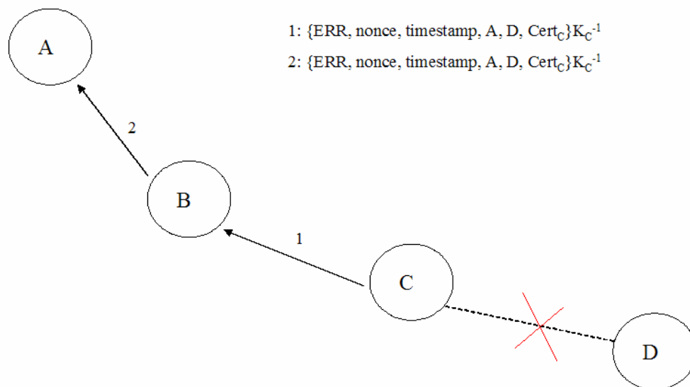
Figure 3. Route maintenance in the ARAN protocol: Error messages are broadcasted without any modification or additional signing by nodes that use the reporting node as a next hop.
