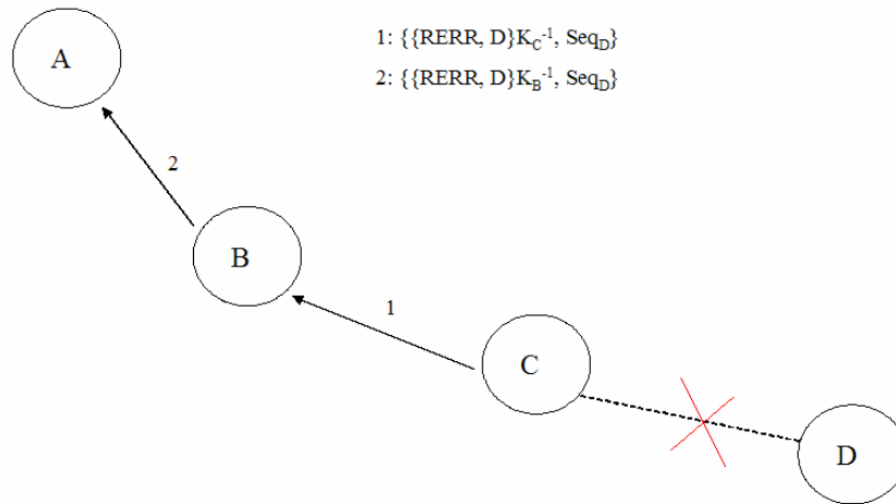
Figure 6. Route maintenance in the SAODV protocol.
